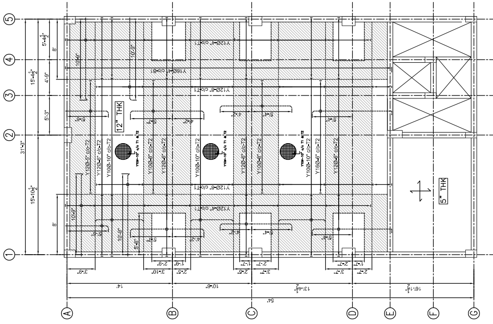
SLAB TOP REINFORCEMENT PLAN
