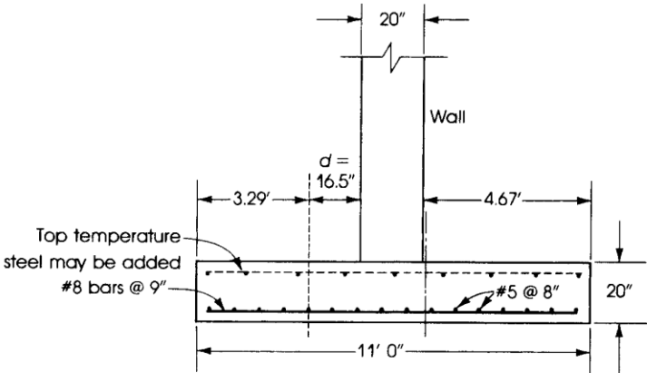
Figure 13.16 Example 13.1: Wall footing.
